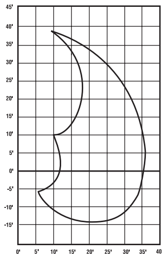
569 SM/569 SM/EHC Pluma de 10,9 m (36' 0")
