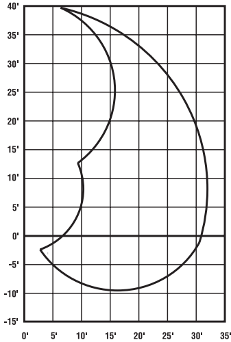
569 SM/569 SM/EHC Pluma de 9,6 m (32' 6")
